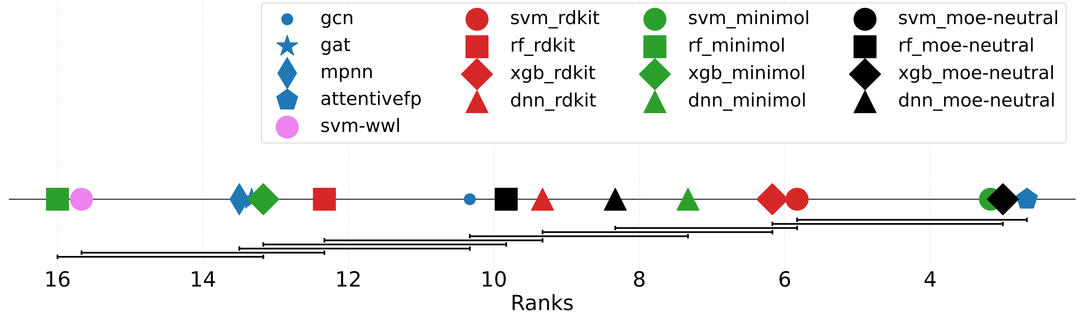
Critical Difference Diagram for Regression Data
